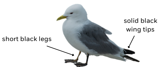
Black-legged Kittiwake
